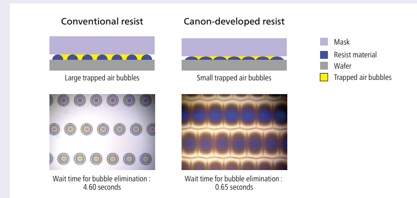
Behavior of resist droplets on a wafer
