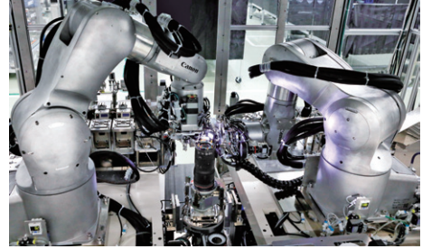
Automated production process for interchangeable lenses
